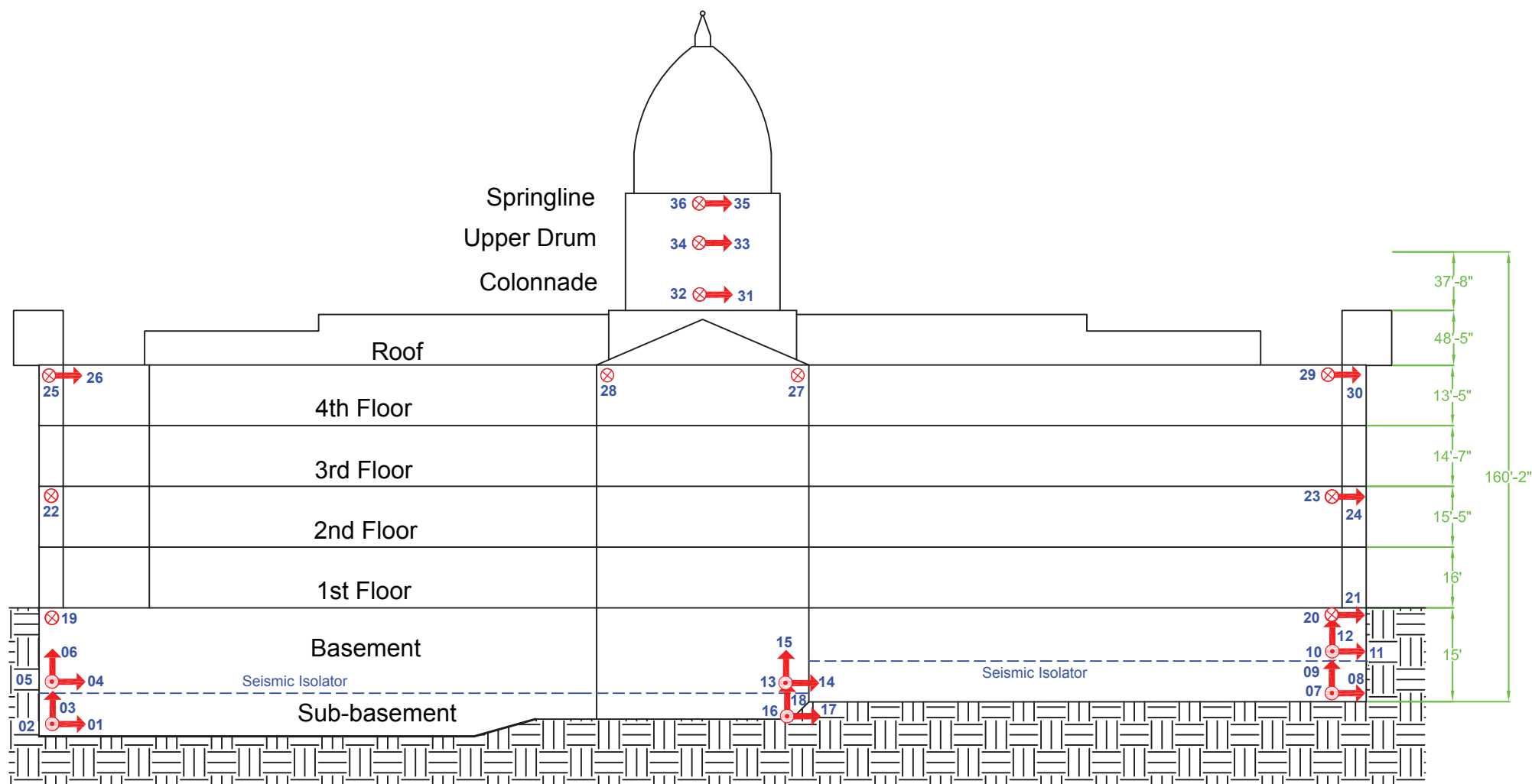
Elevation View Looking Reference North
