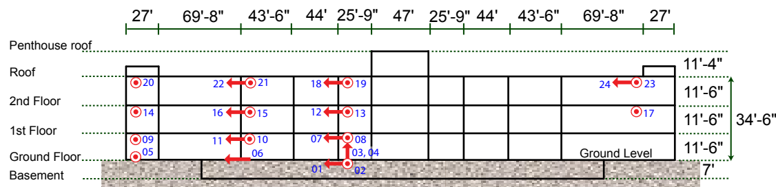
Elevation View Looking Reference North
