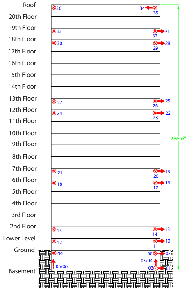
Elevation View Looking Reference North
