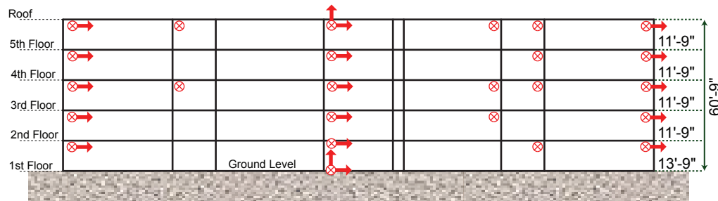
Elevation View Looking Reference North
