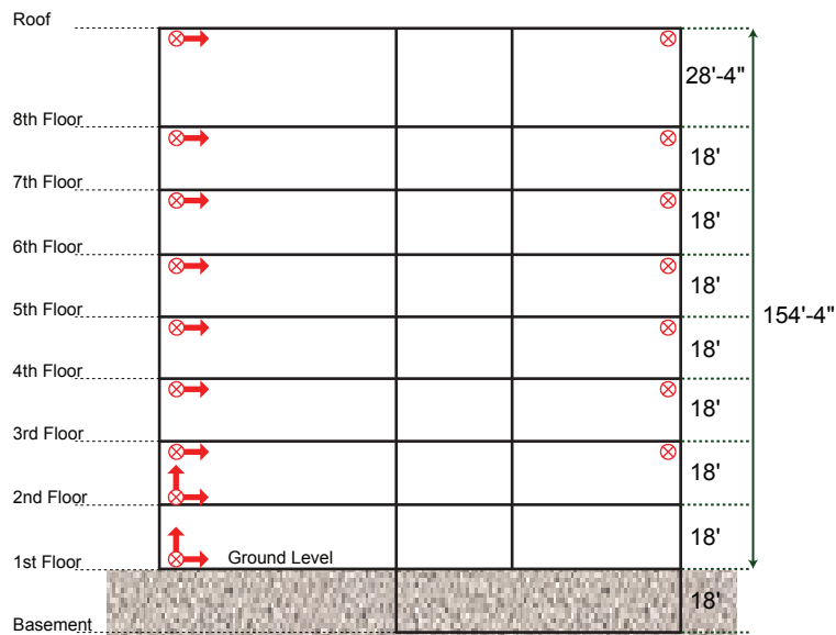
Elevation View Looking Reference North
