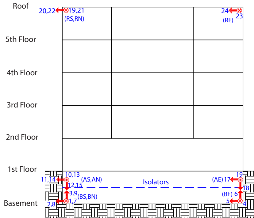
Elevation View Looking Reference North
