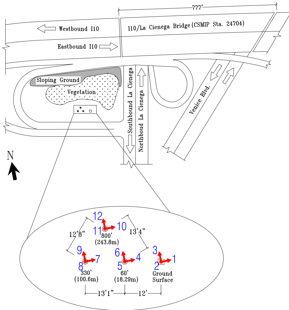
Enlarged Plan
