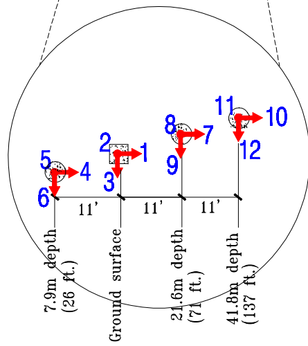
Enlarged Plan
