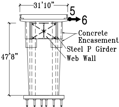
W/E Elevation Pier 15
