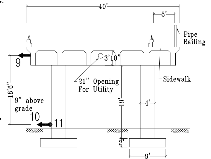
Section A - A' @ Bent 3
