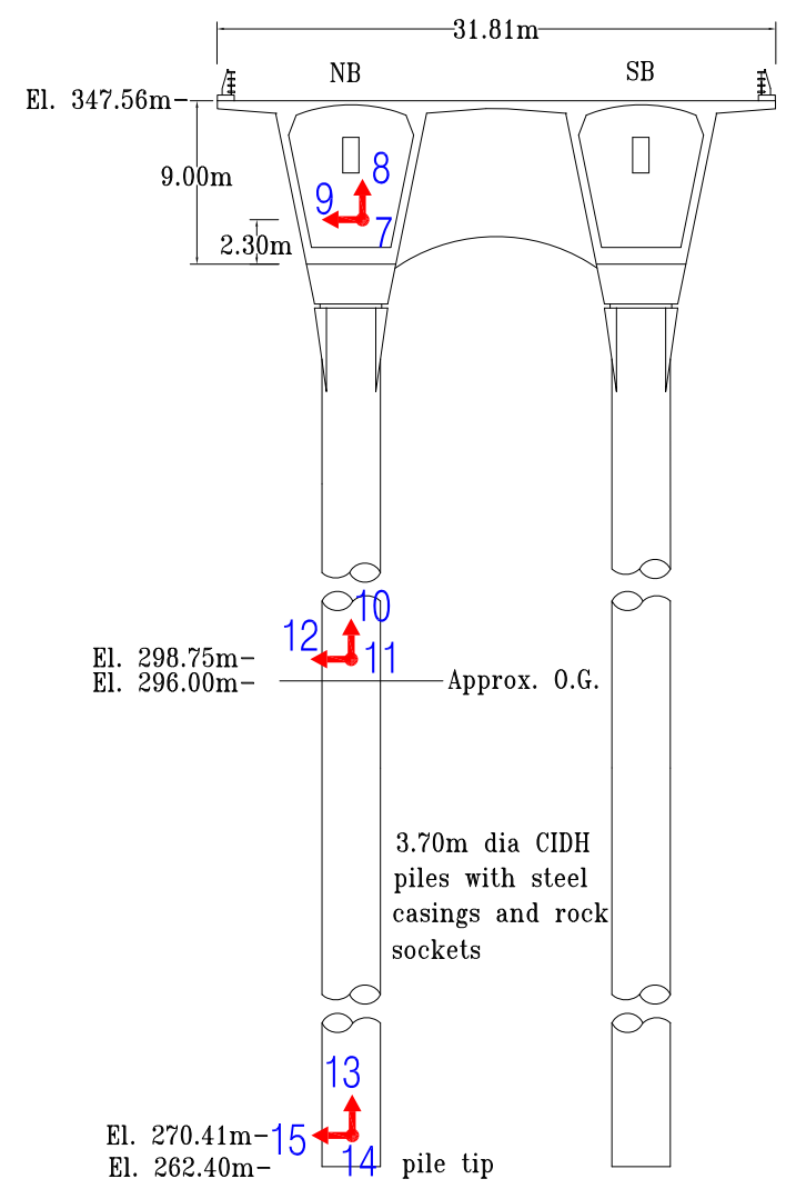
Section A-A' at Pier 4
