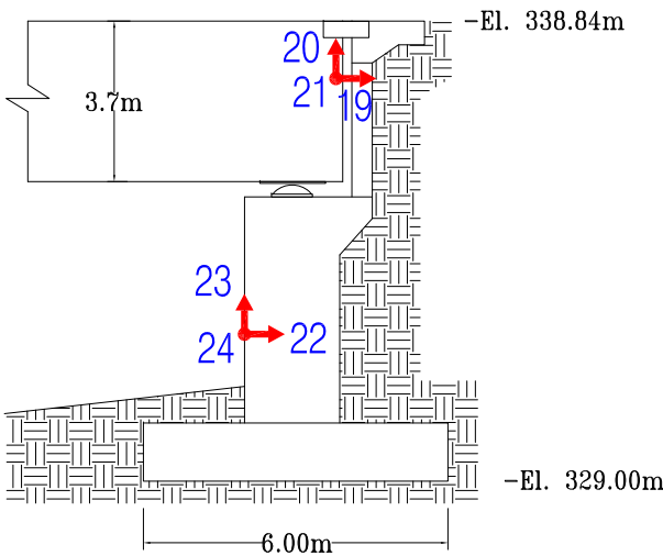
Section of Abutment 6
