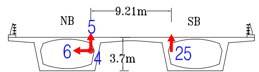
Section B-B' at Midspan between Piers 3 & 4
