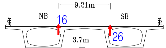
Section C-C' at Midspan between Piers 4 & 5
