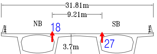
Section D-D' at Midspan between Piers 5 & Abutment 6
