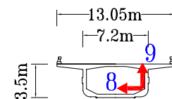
Section at Midspan between Piers 2 & 3
