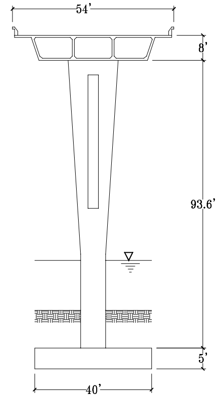
Section A-A' at Bent 3
