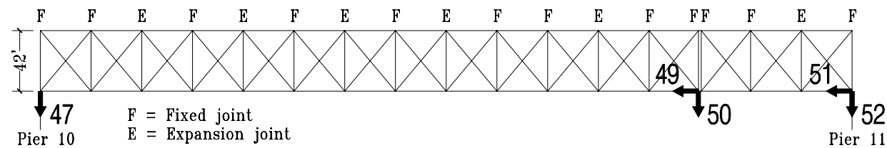
Plan - Pier 10 through Pier 11
