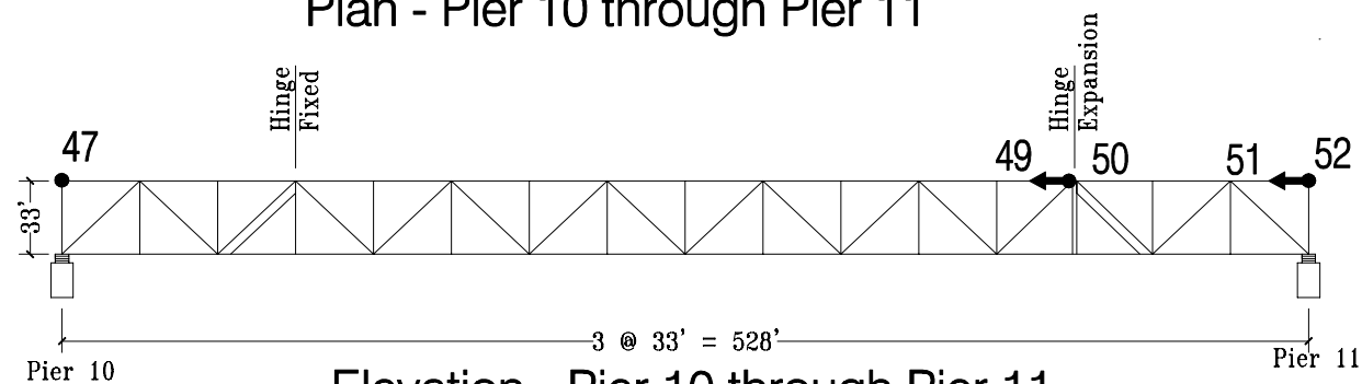
Elevation - Pier 10 through Pier 11
