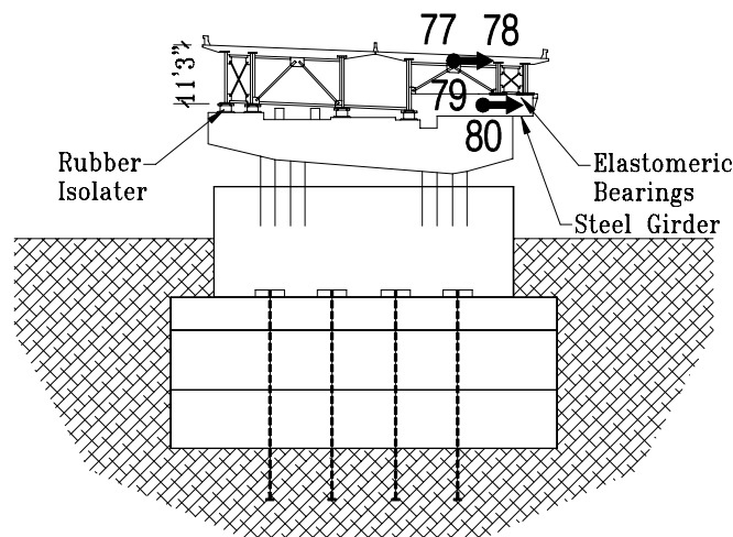
E/W Section at Pier 18
