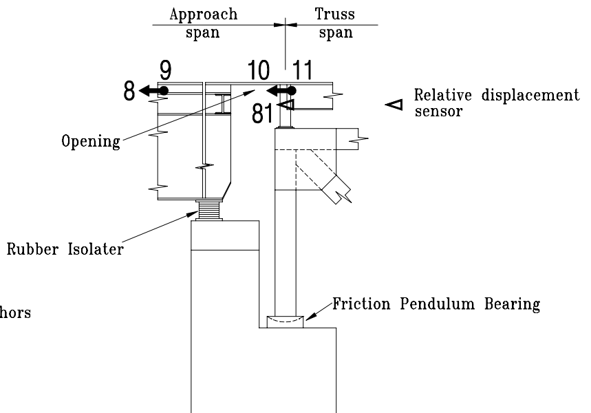
N/S Elevation at Pier 3
