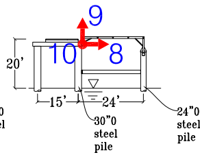
Section C-C'
