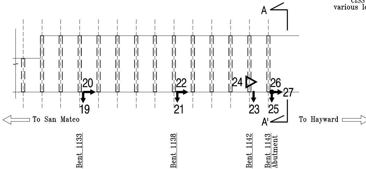
Deck Level Plan
