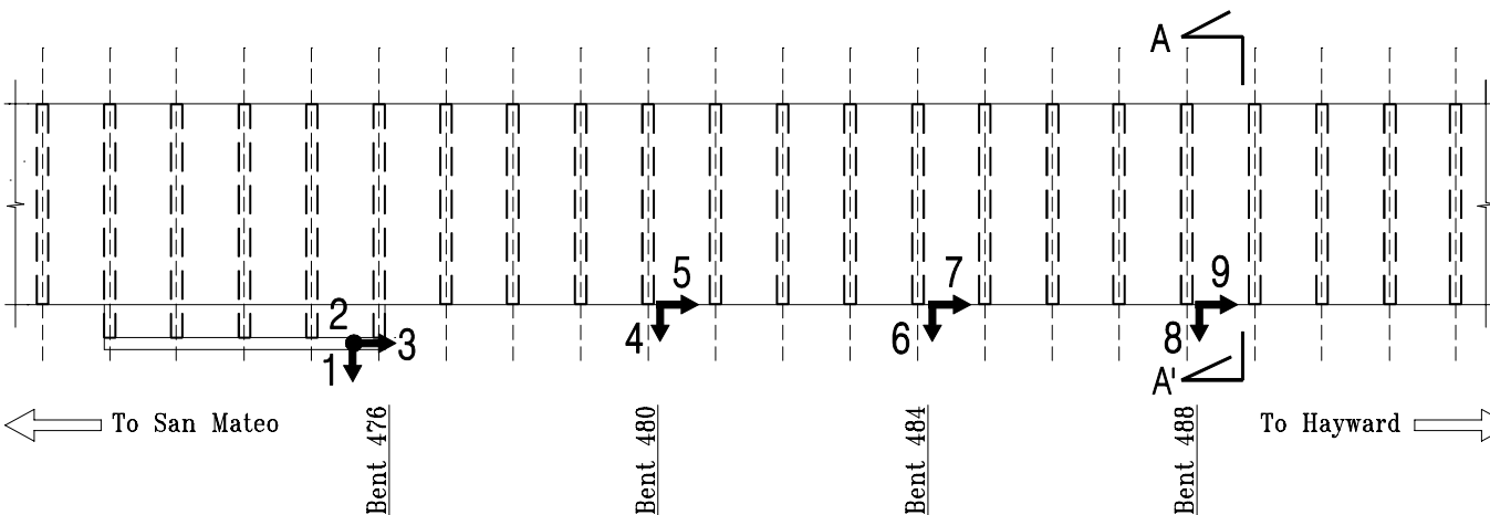
Deck Level Plan
