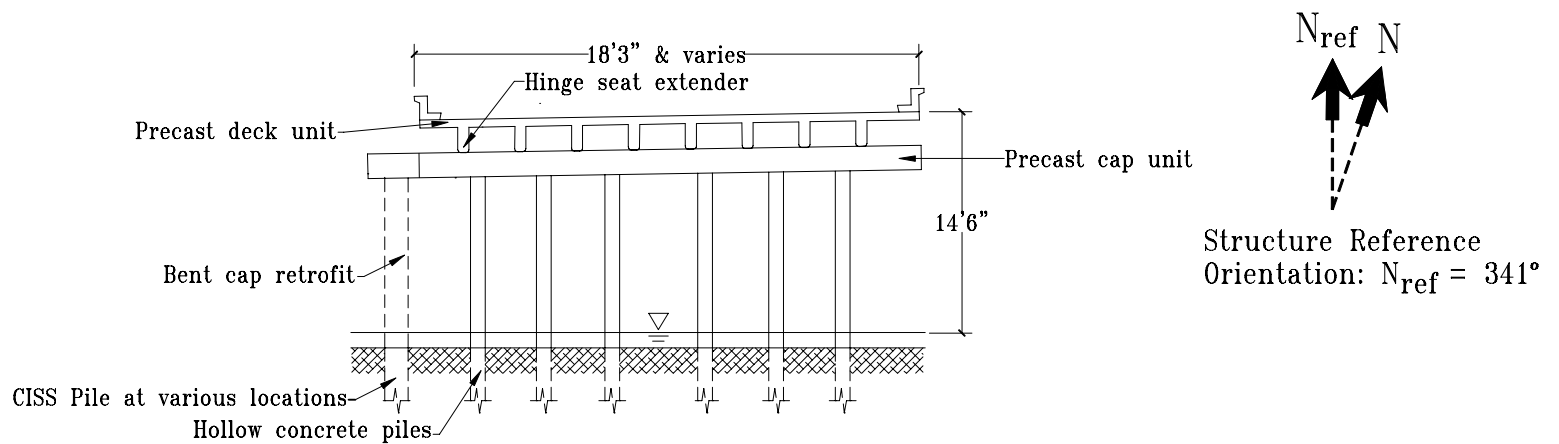
Typical Section
