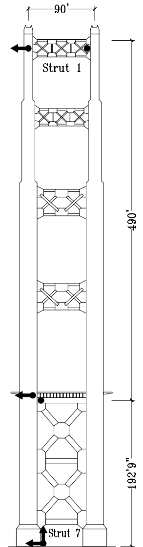
W/E Elevation of Marin (North) Tower
