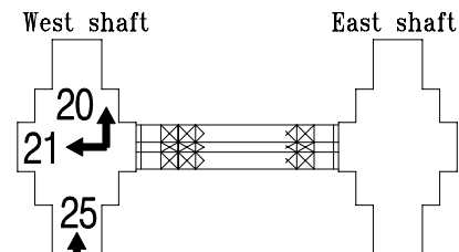
Roadway Level Plan
