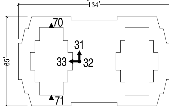
Base Level Plan
