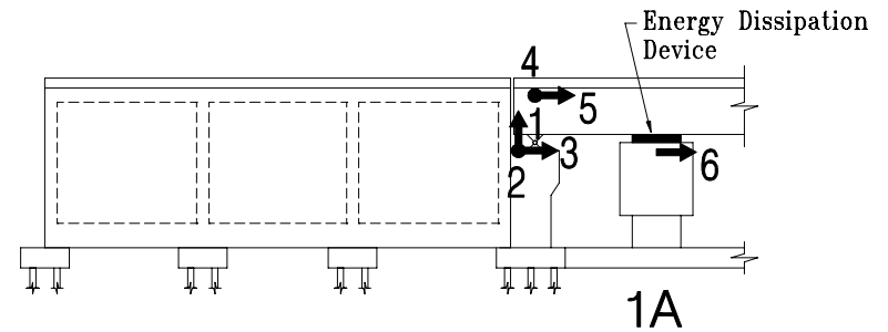
South Elevation - Piers 1 & 1A
