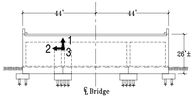
S/N Section - Pier 1
