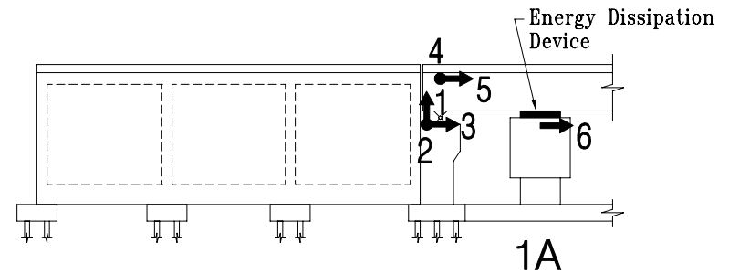
South Elevation - Piers 1 & 1A
