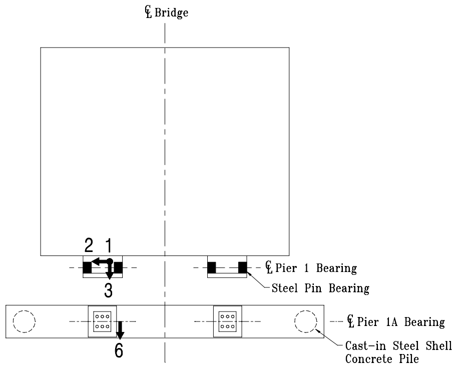
Plan - Piers 1 & 1A
