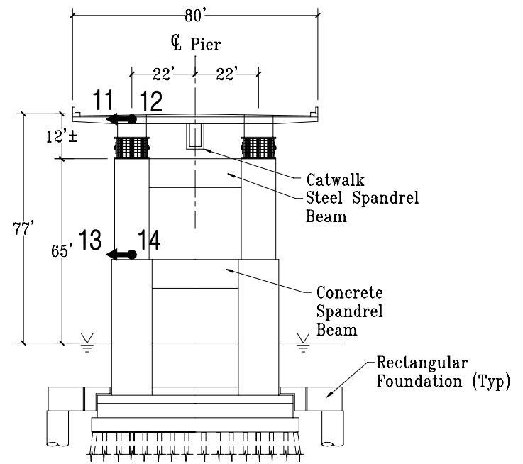
S/N Section Pier 9
