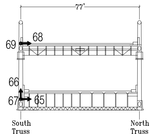
Midspan Between Towers W5 and W6
