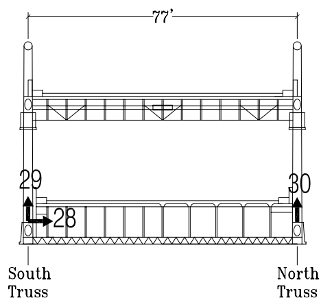
Midspan Between Towers W2 and W3
