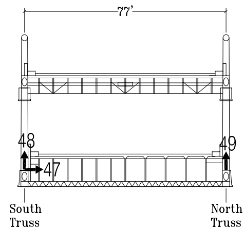
Midspan Between Tower W3 and Pier W4
