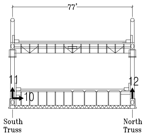
Midspan Between Pier W1 and Tower W2
