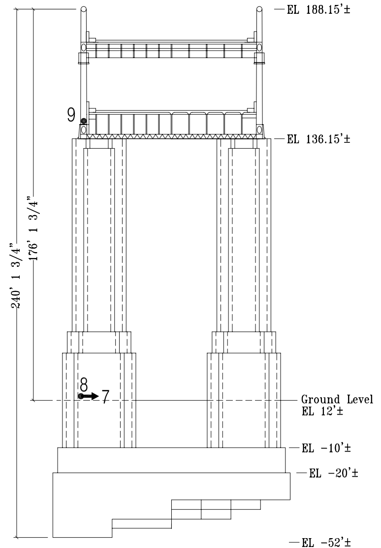
East Elevation at Pier W1
