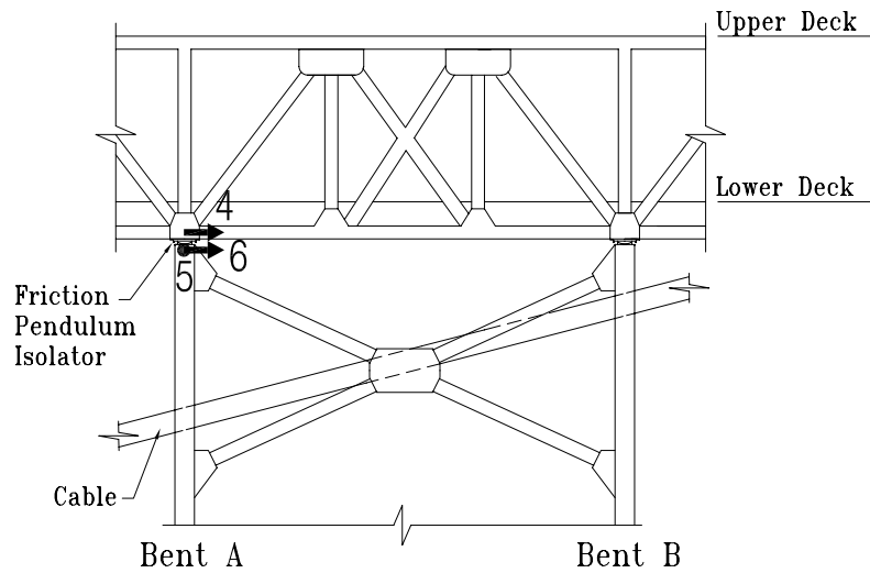
South Elevation of South Legs of Bents A and B
