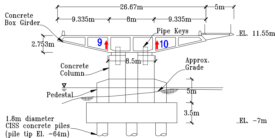
N/S Section at Pier E18 (Eastbound)
