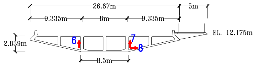
N/S Section at Midspan between Piers E17 and E18 (Eastbound)
