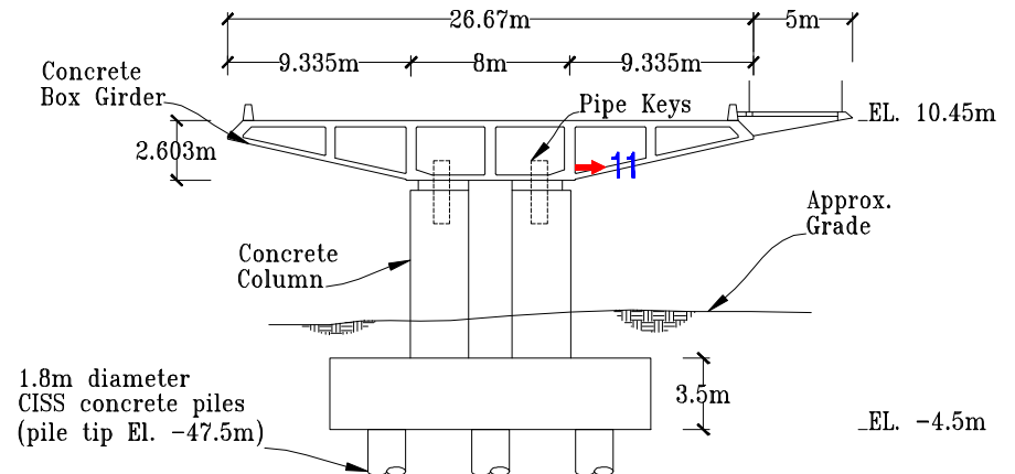
N/S Section at Pier E19 (Eastbound)
