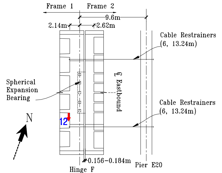
Deck Plan at Hinge F (Eastbound)
