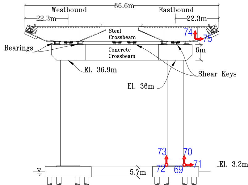
N/S Section at Pier E2
