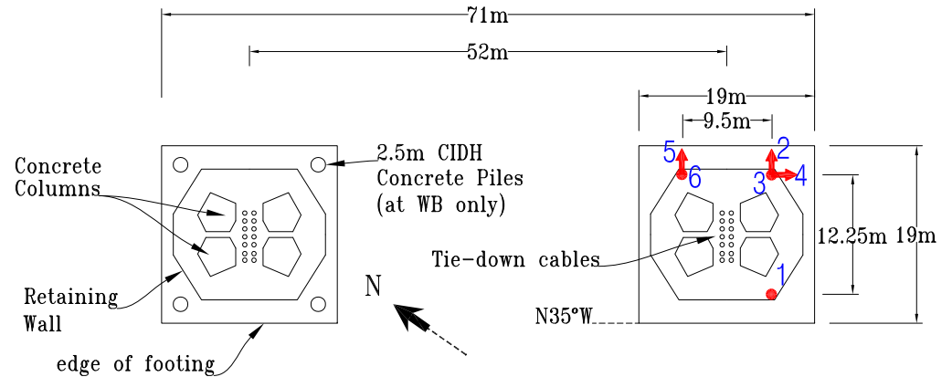
Top of Footing Plan at Pier W2
