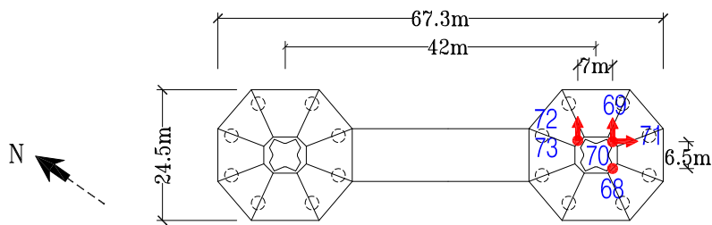
Footing Plan at Pier E2
