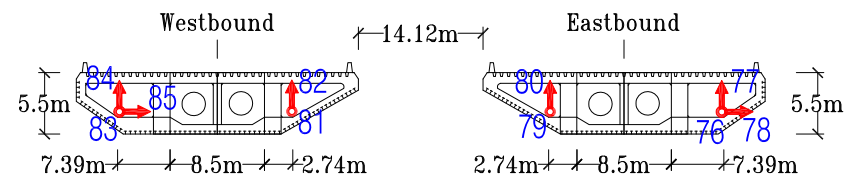
Section A-A' at Hinge A (Panel Point 127.5)
