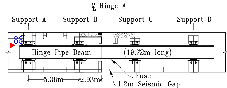
Section B-B' at Hinge A (EB)
