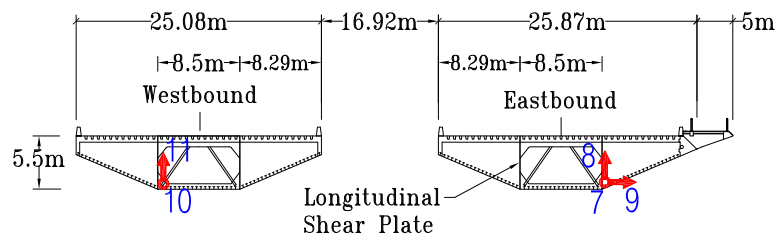
Section A-A' at Hinge K (Panel Point 8)
