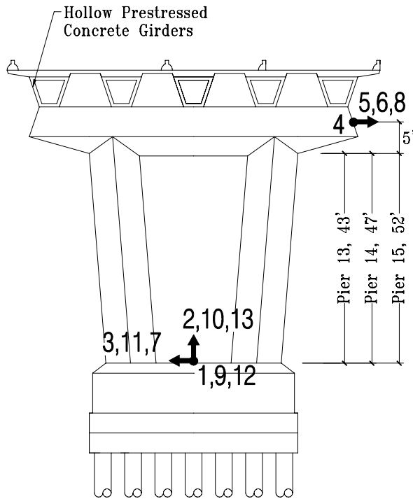
N/S Section @ Piers 13, 14, 15
