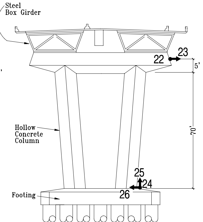
N/S Section @ Pier 21
