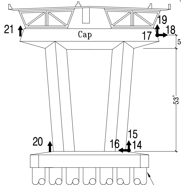
N/S Section @ Pier 17
