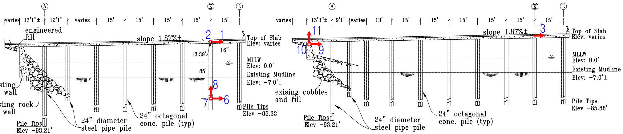
Section A-A' at Line 12
