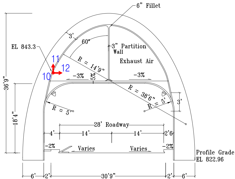
Section C-C' Station 223+61
