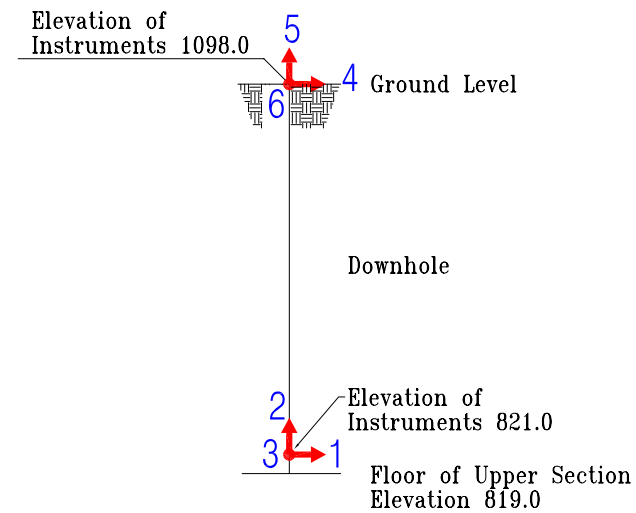
Section D- D' at Downhole
