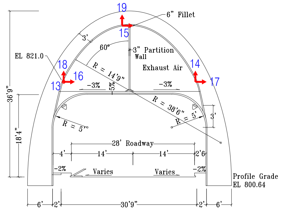
Section B-B' Station 218 + 03
