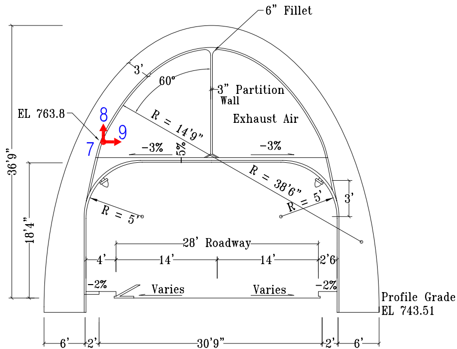
Section A-A' Station 207 + 63
