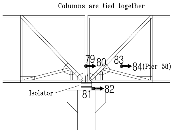
W/E Elevation at Pier 55 (Pier 58 Similar)
