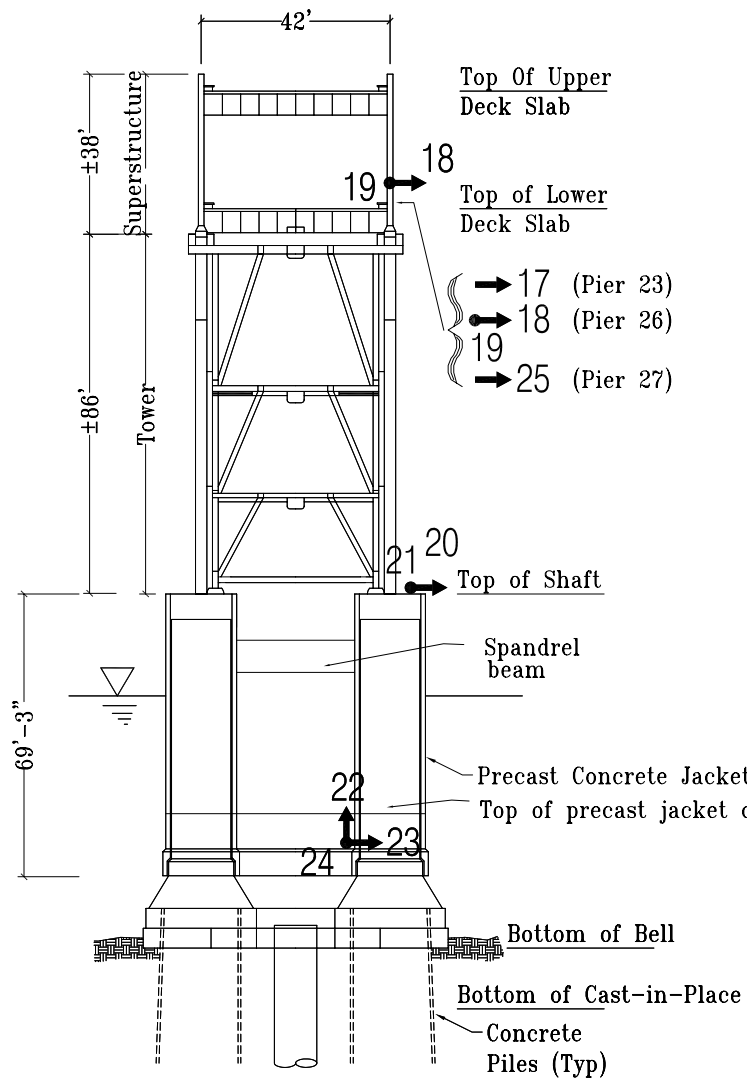
N/S Section at Pier 26 (Pier 23 & 27 Similar)
