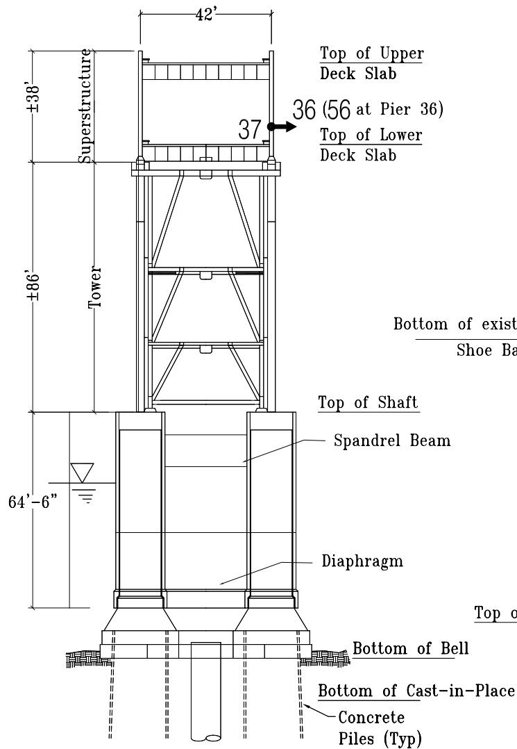
N/S Section at Pier 33 (Pier 36 Similar)
