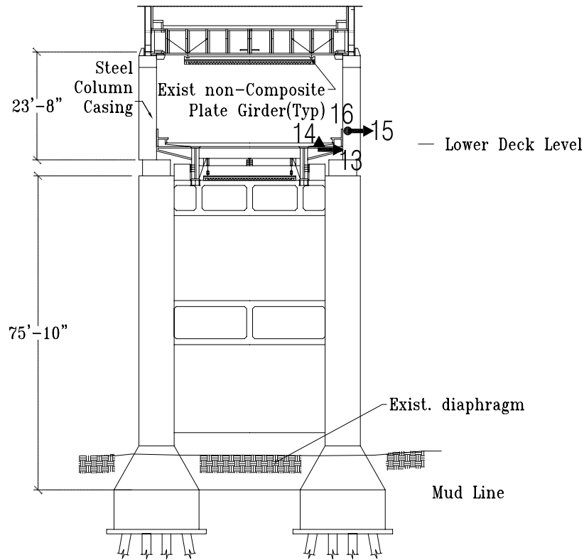
N/S Section at Pier 19 (Plate Girder Side)
