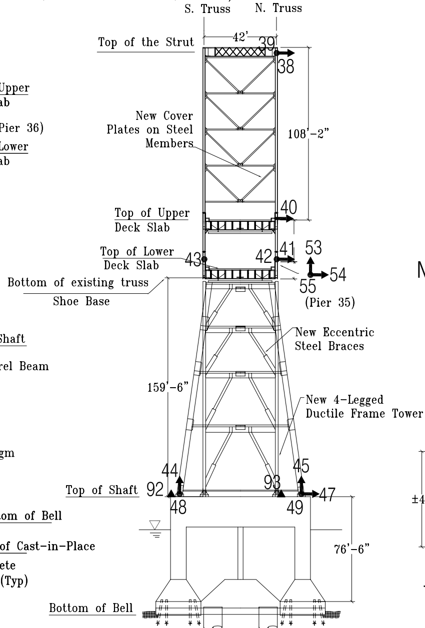
N/S Section at Pier 34 (Pier 35 Similar)
