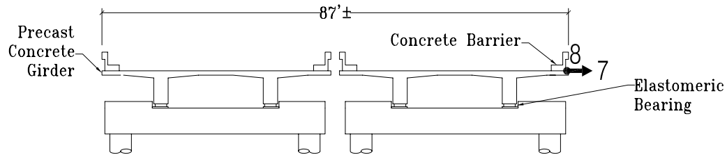
N/S Section at Bent 1
