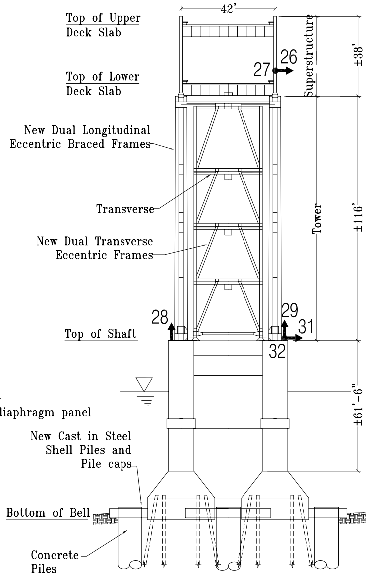
N/S Section at Pier 30
