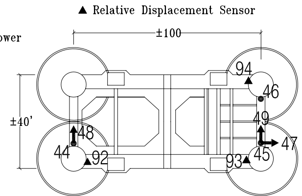
Top of Shaft Plan at Pier 34
