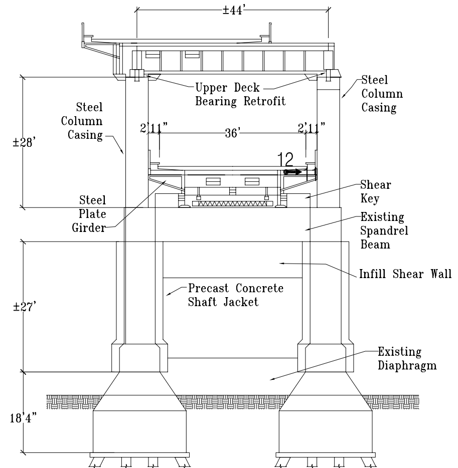
N/S Section at Pier 10
