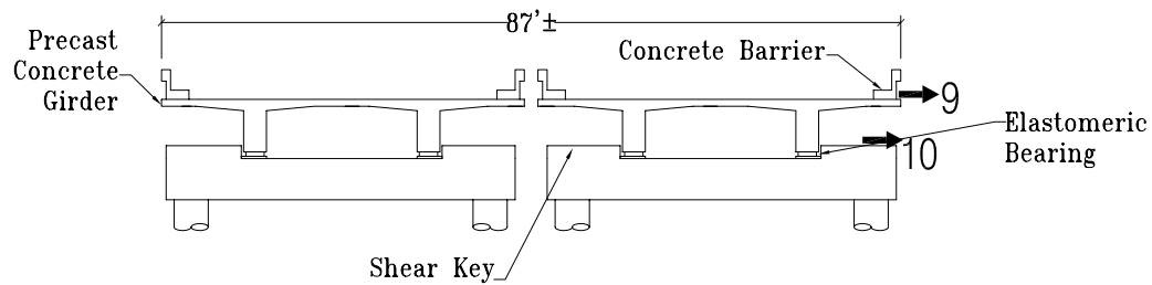
N/S Section at Bent 5
