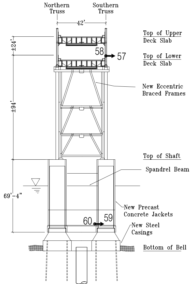
N/S Section at Pier 39
