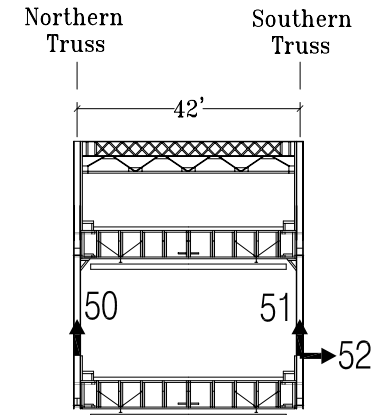
Midspan Section Between Piers 34 and Pier 35
