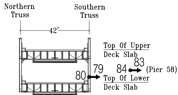
N/S Section at Pier 55 (Pier 58 Similar)
