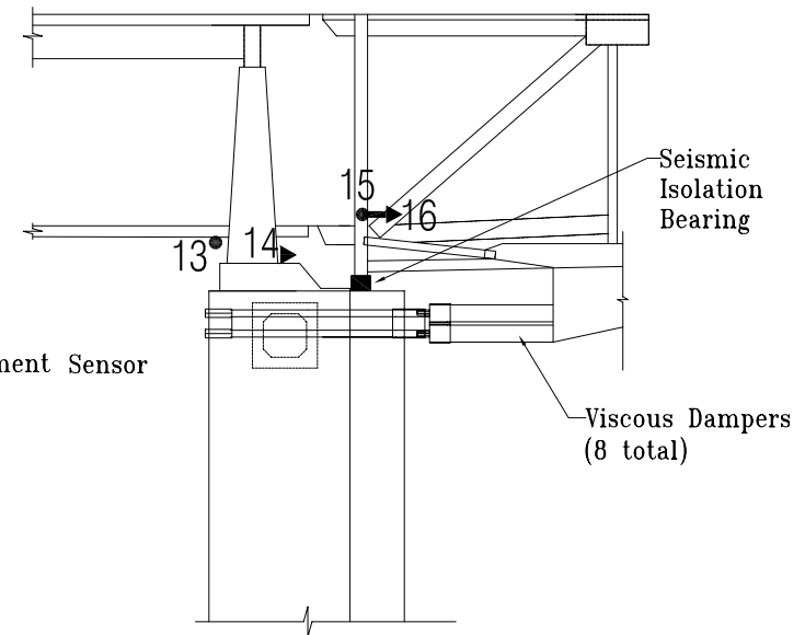
South Elevation at Pier 19
