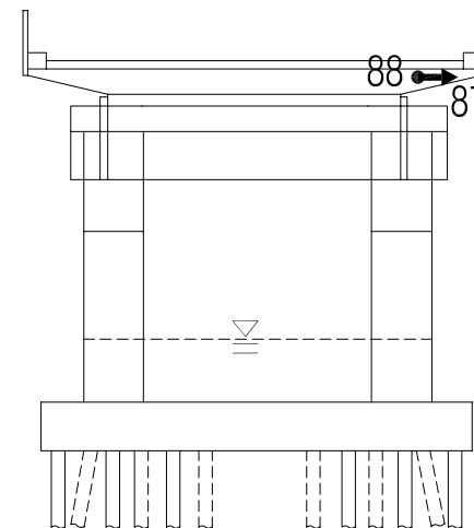
N/S Section at Pier 76R
