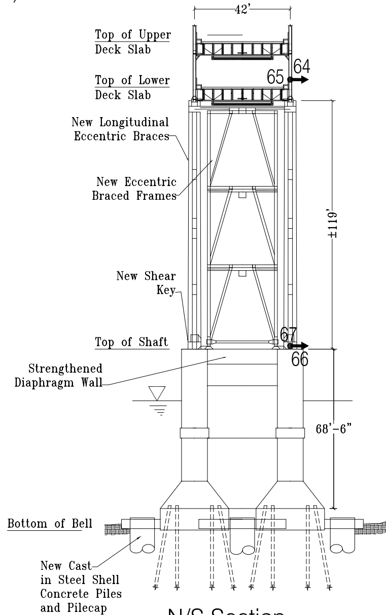
N/S Section at Pier 44
