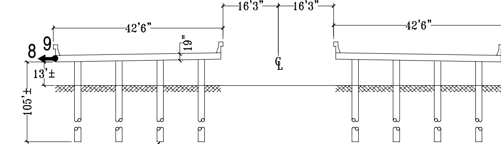
Section A-A' at Bent 13
