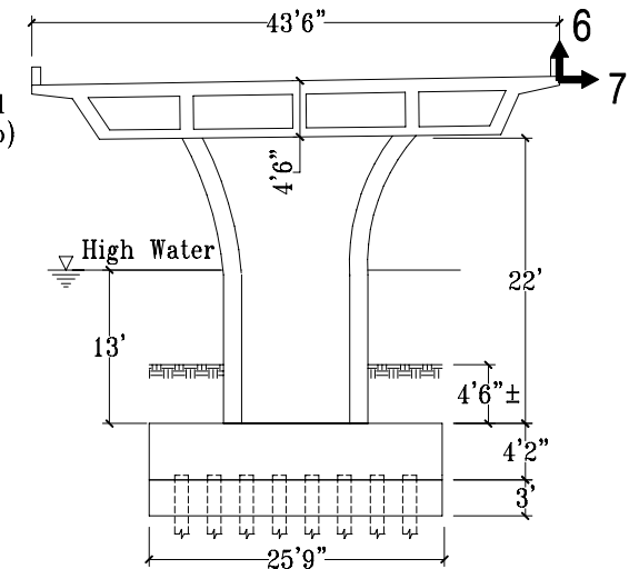
Section A-A' at Pier 3
