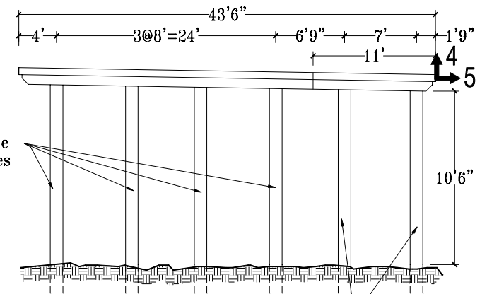
N/S Section @ Bent 4
