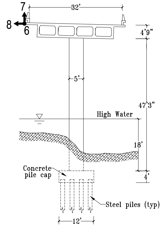
Section A-A' at Bent 3
