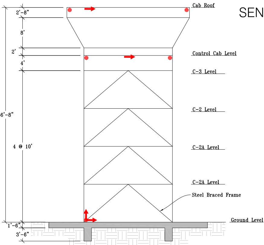
South Elevation
