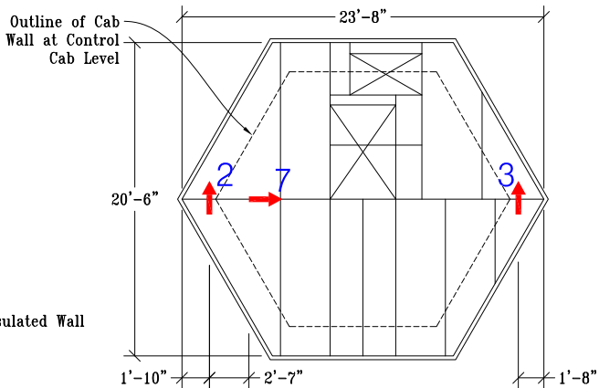
Cab Roof Plan
