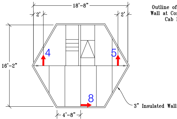
Control Cab Level Plan
