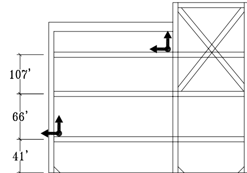
North Elevation
