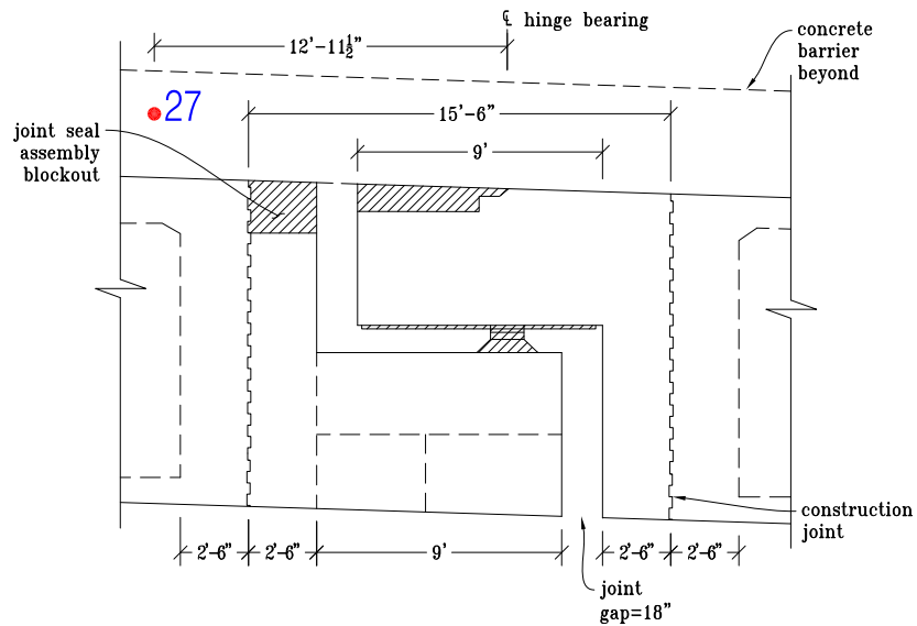
S/N Section at Hinge 6 (North of Bent 20)
