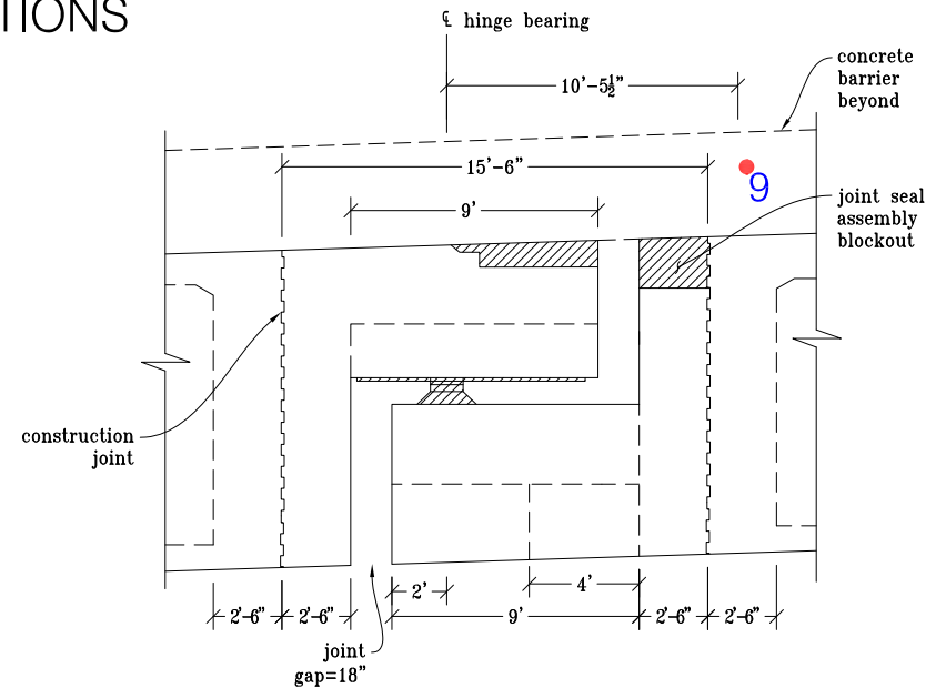
S/N Section at Hinge 3 (South of Bent 11)
