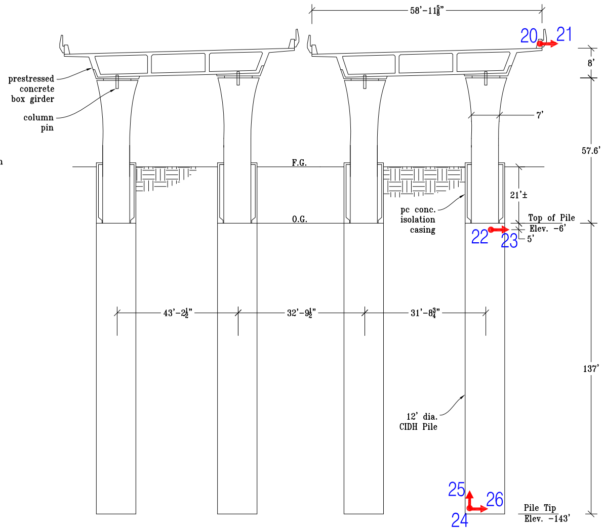
S/N Section at Hinge 5 (North of Pier 16)
