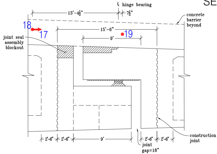
S/N Section at Hinge 5 (North of Pier 16)
