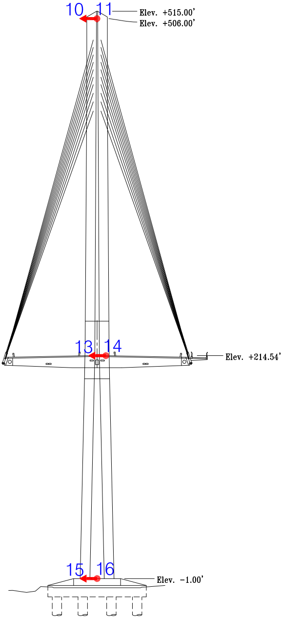
N-S Elevation @ Tower 16
