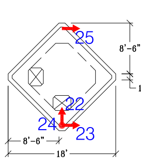
Section @ Tower 17 (Elev. +506.00')
