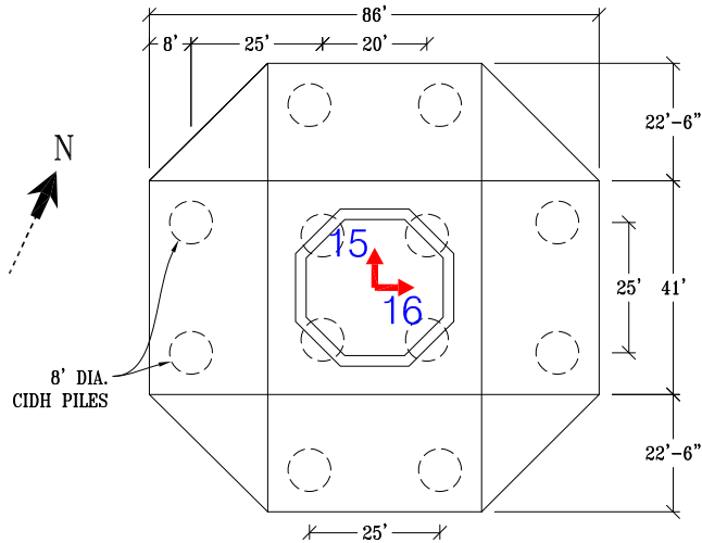
Pile Cap @ Tower 16 (Elev. -1.00')
