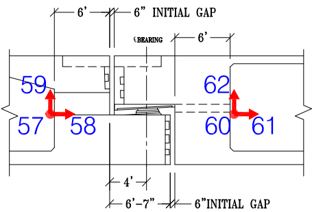
Section @ Hinge 6B
