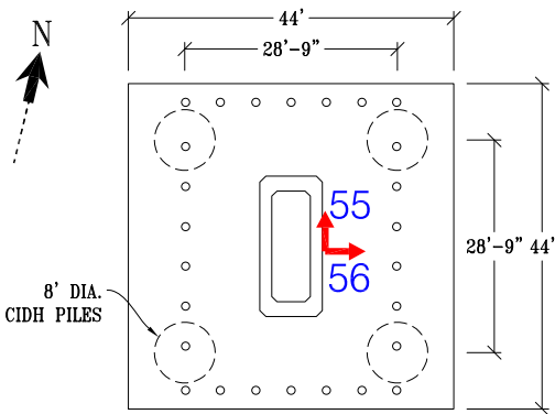
Pile Cap @ Bent 22
