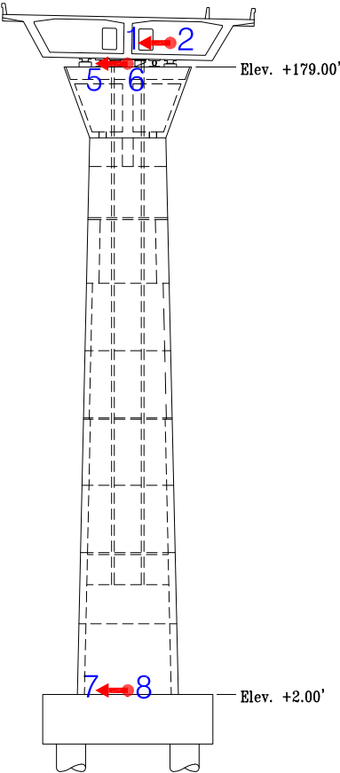
N-S Elevation @ Bent 15
