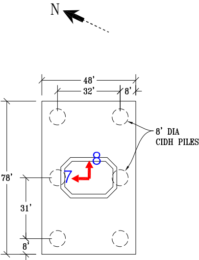
Pile Cap @ Bent 15
