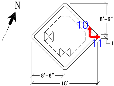
Section @ Tower 16 (Elev. +506.00')
