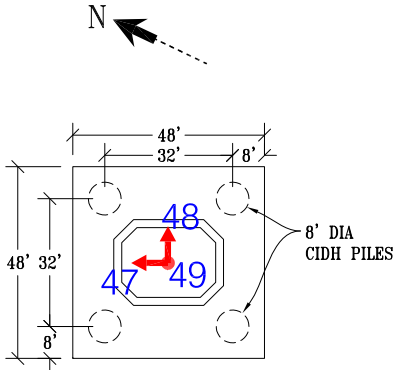
Pile Cap @ Bent 18
