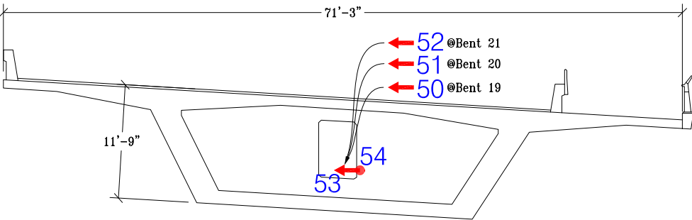
N - S Section @ Bent 22 (Bent 19, 20, 21 Similar)
