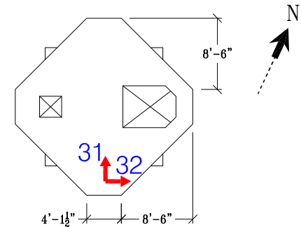
Section @ Tower 17 (Elev. +214.54')
