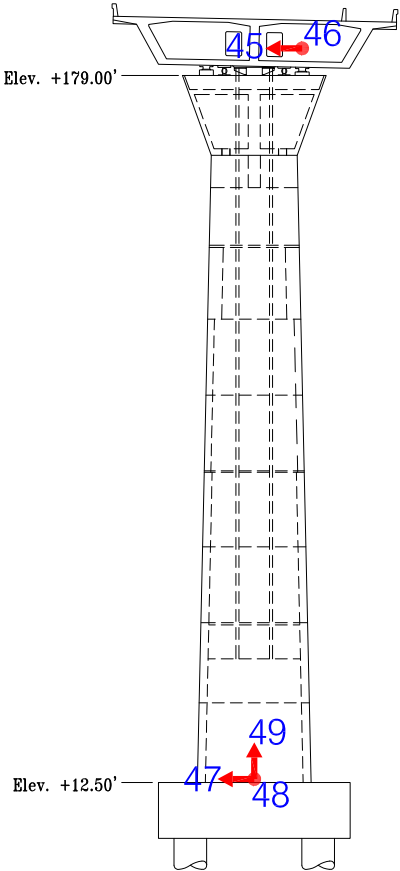
N-S Elevation @ Bent 18
