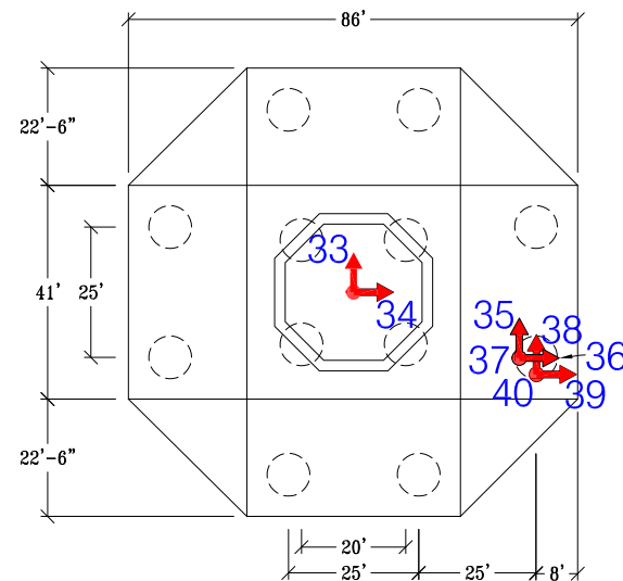
Pile Cap @ Tower 17 (Elev. +20.00')
