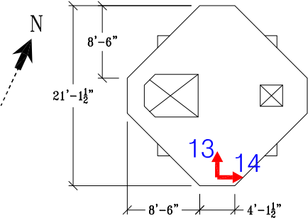
Section @ Tower 16 (Elev. +214.54')
