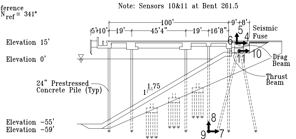
Section A-A' at Bent 261
