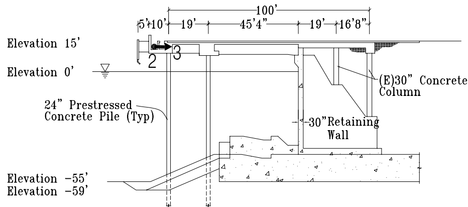
Section B-B' at Bent 260a
