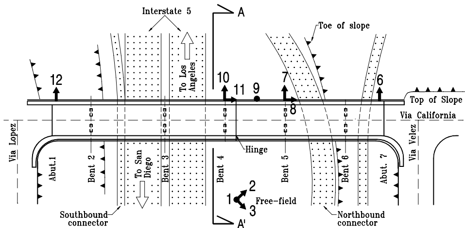
Deck Level Plan
