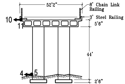
Section A-A' at Bent 4
