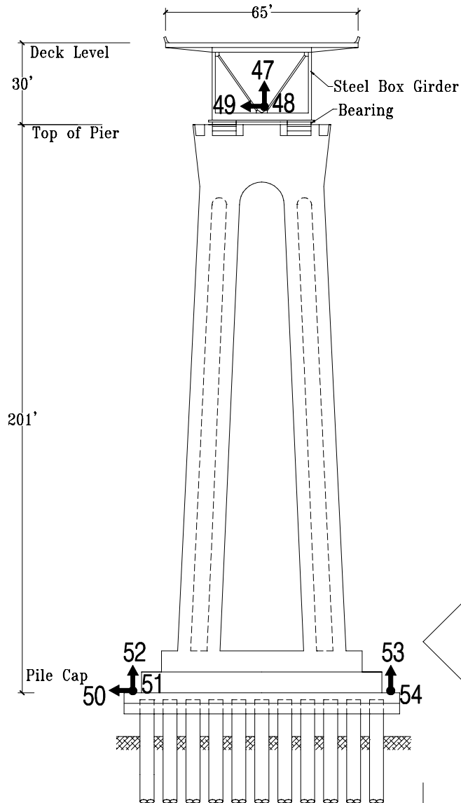
Section at Pier 19
