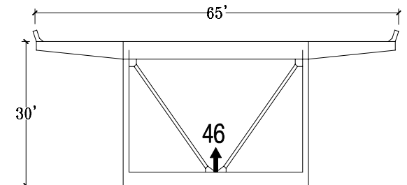
Midspan Section between Piers 18 & 19
