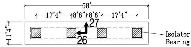
Top of Pier Plan
