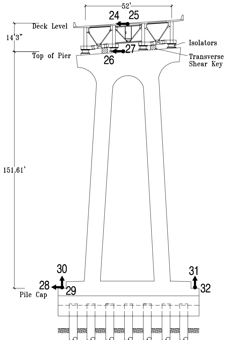
Section at Pier 14
