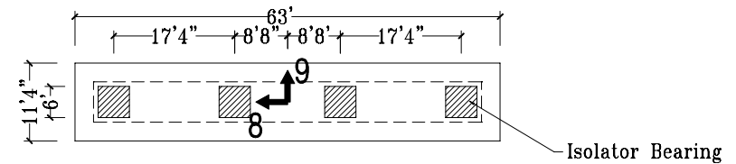
Top of Pier 5 Plan
