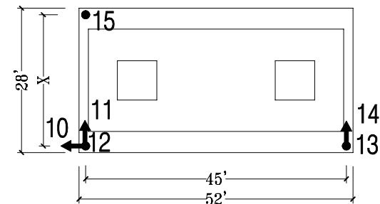
Pile Cap of Pier 5 Plan
