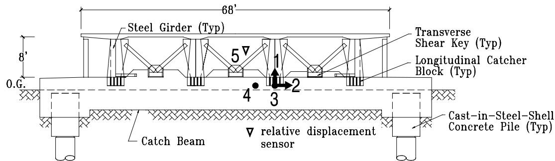
Elevation at Abutment 1
