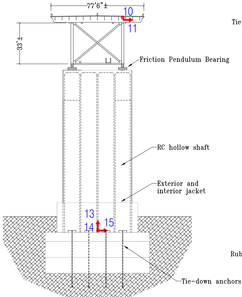
E/W Section at Pier 3
