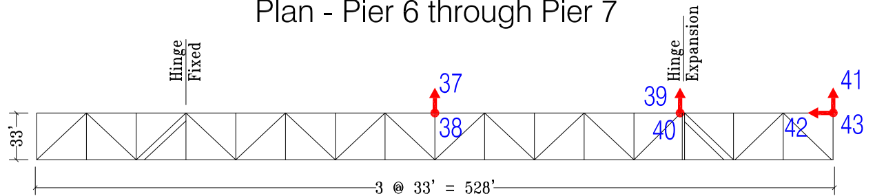
Elevation - Pier 6 through Pier 7
