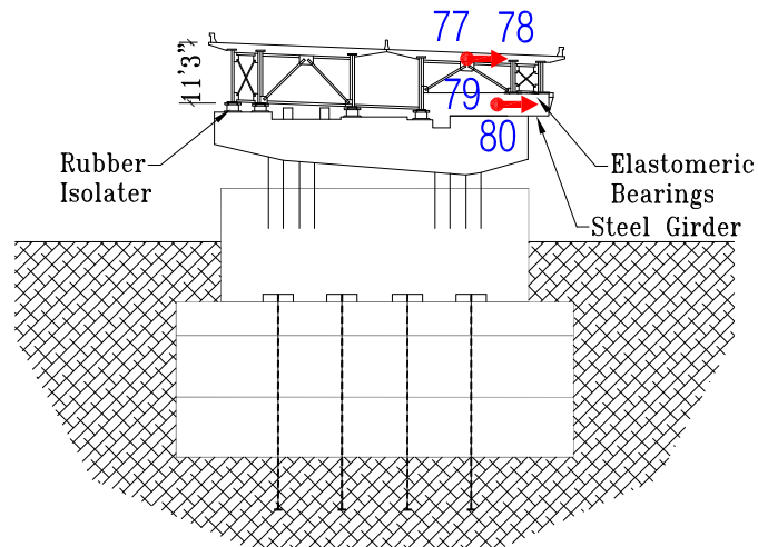
E/W Section at Pier 18
