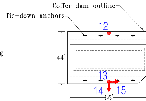
Footings at Pier 3
