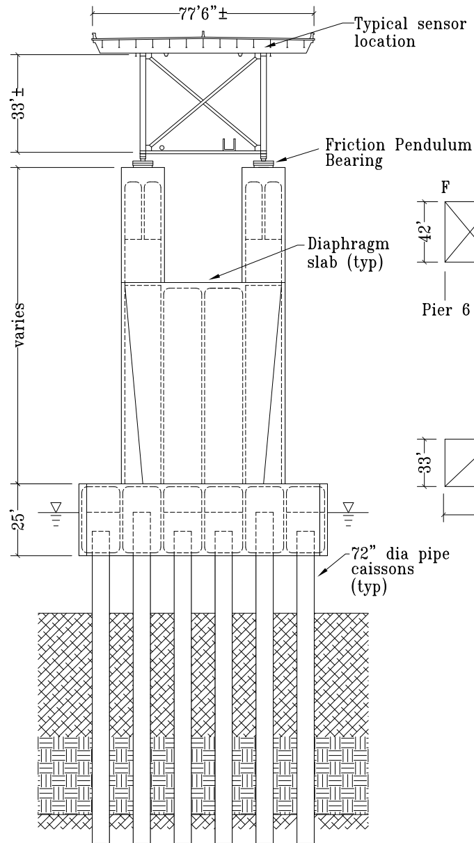
E/W Section at Piers 7-11
