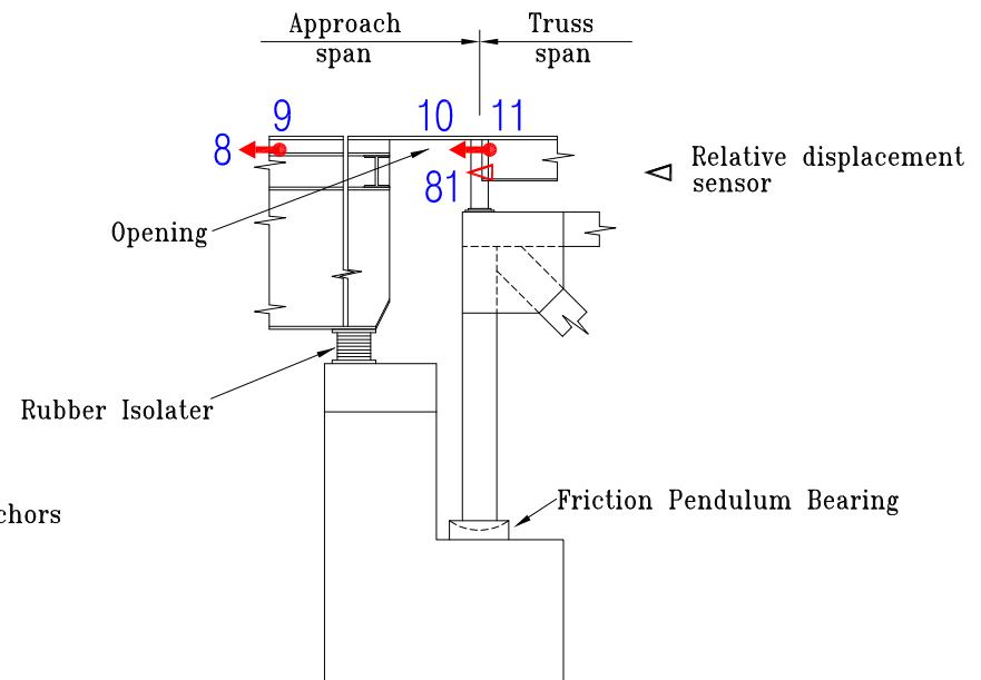
N/S Elevation at Pier 3
