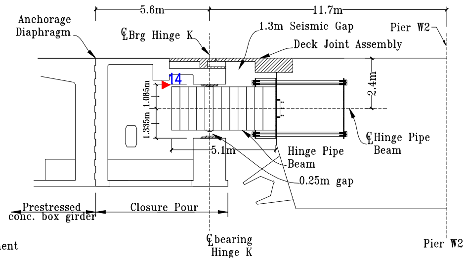
Section B-B' at Hinge K - Westbound (Similar for Sensor 25)
