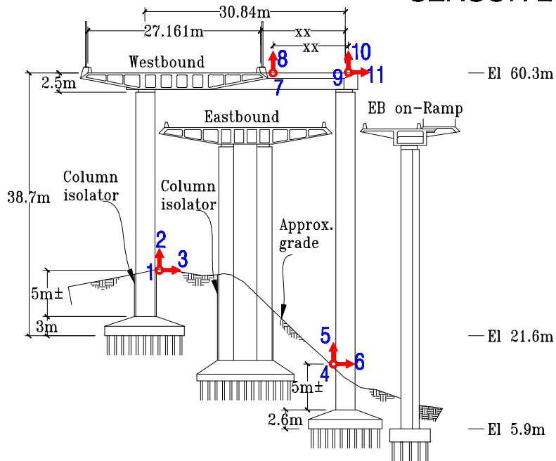
N/S Elevation at Bent W7
