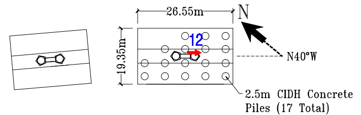
Footing Plan at Bent W4
