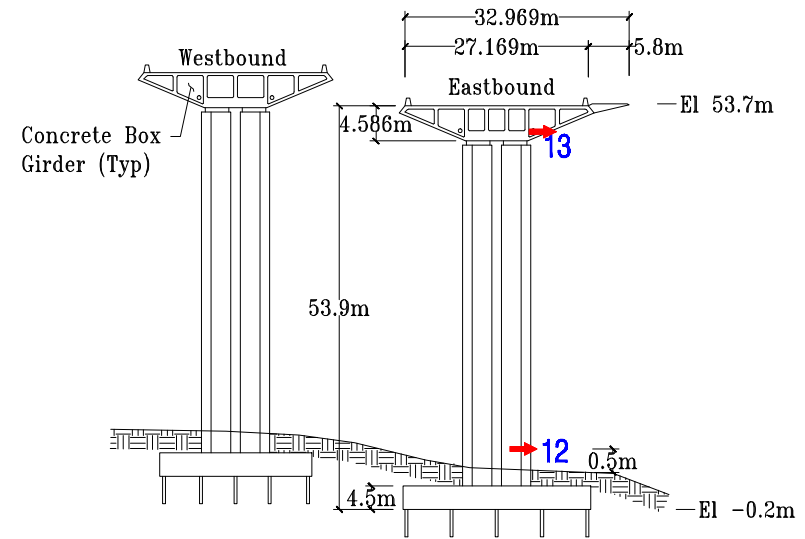
N/S Elevation at Bent W4
