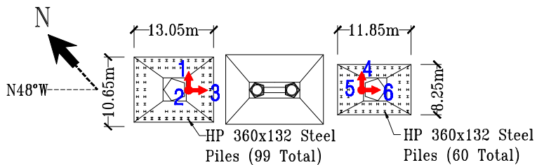
Footing Plan at Bent W7
