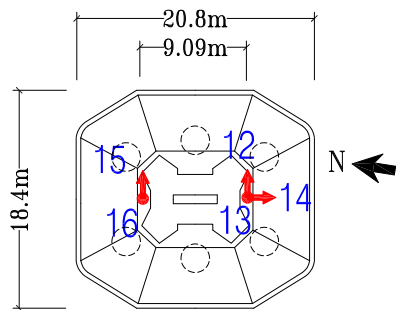
Footing Plan at Pier E5E
