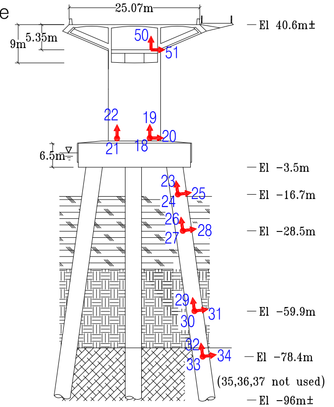
N/S Elevation at Pier E6E
