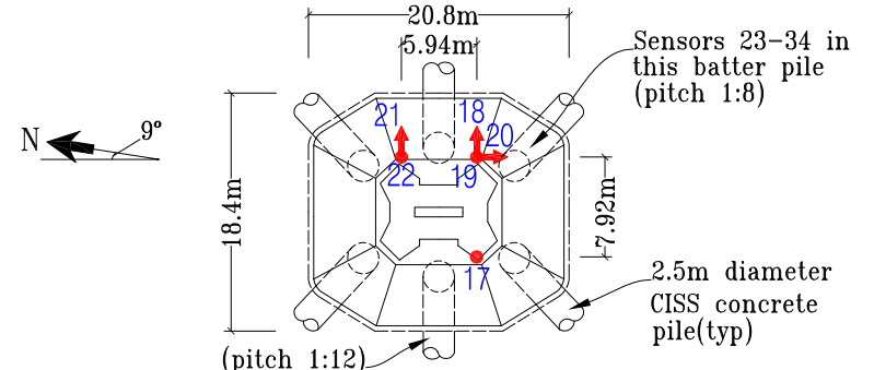
Footing Plan at Pier E6E
