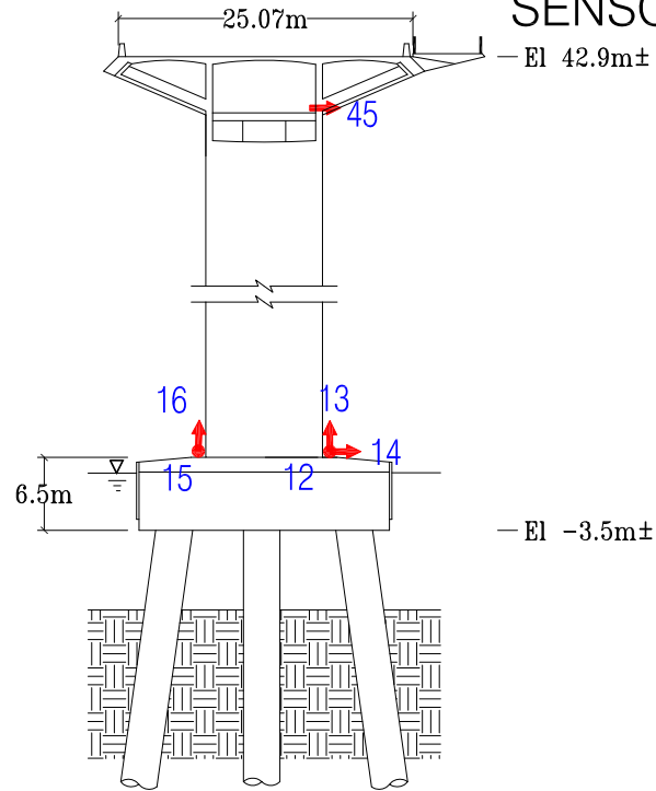
N/S Elevation at Pier E5E
