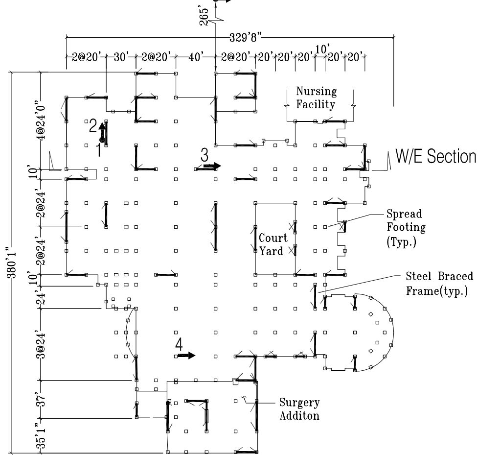
Ground Floor/Foundation Plan
