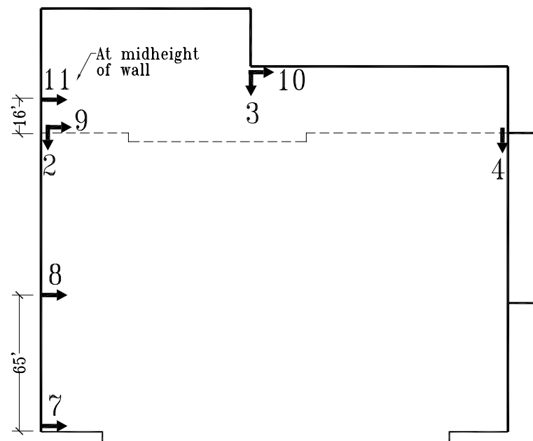
Roof Plan
