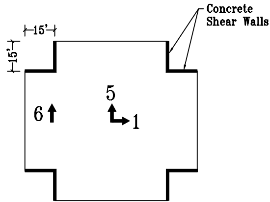
5th Floor Plan
