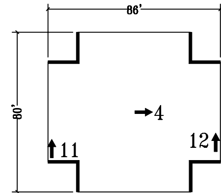
Roof Plan
