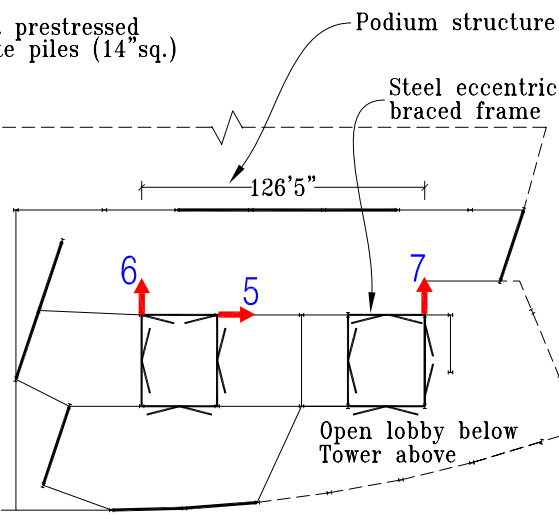
Level P5 Plan
