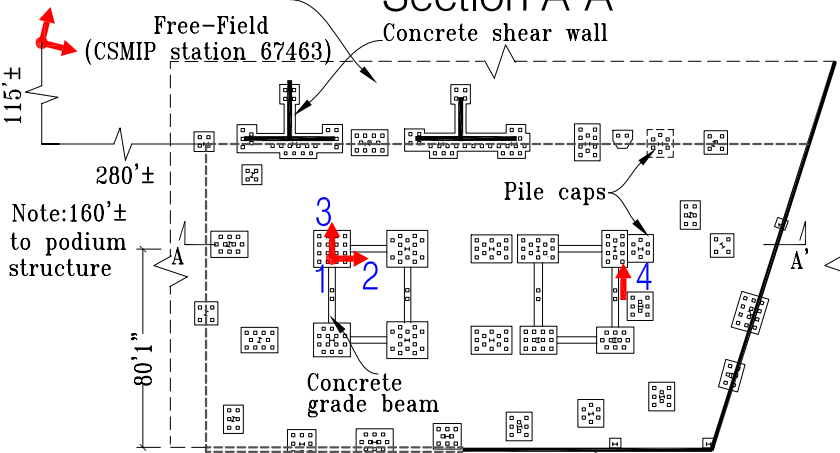
Level P1 Plan
