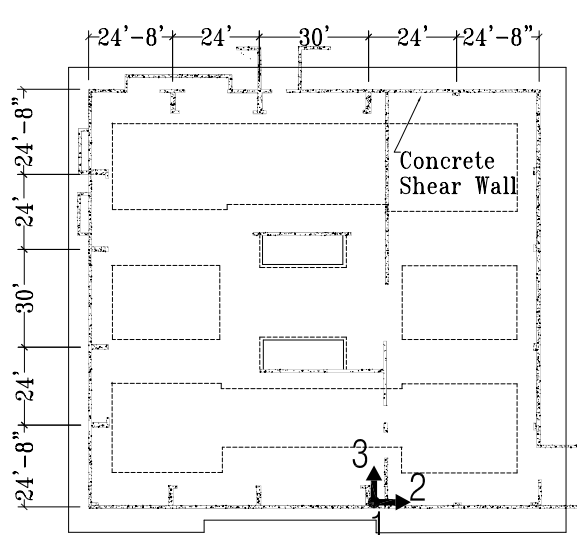
Basement Plan
